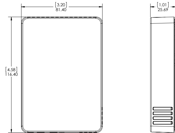
T5100 standard enclosure
