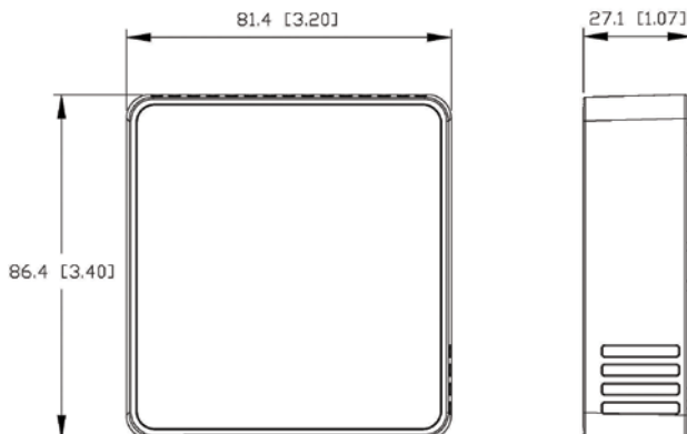
T5100-EC smaller Euro enclosure
